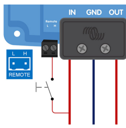
d) Controllo BMS tramite pin H
