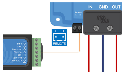
Collegamenti on/off remoti
